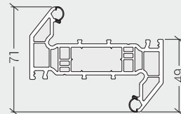
LCW9022 Zero|90 Transom Z
