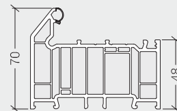
LCW9017 Zero|90 Large Outer Frame
