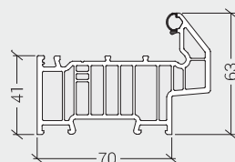
LCW9014 Zero|90R Rebated Frame OF
