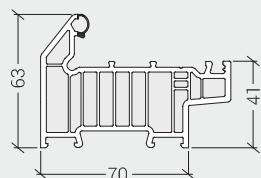
LCW9013 Zero|90R Rebated Frame BF
