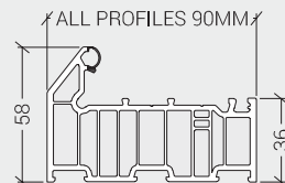
LCW9012 Zero|90 Outer Frame
