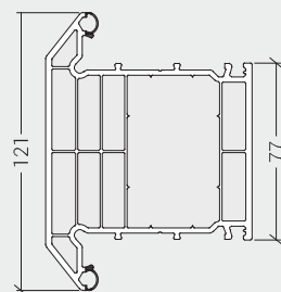
LCW9029 Zero|90 Midrail
