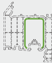
LSR036 / LSR036P Zero|90 Door Sash Reinforcement
