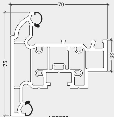
LFS031 80mm Flush Sash
