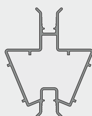
LFS251 80mm 135° Corner joint
