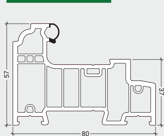
LFS011 80mm Flush Outer Frame
