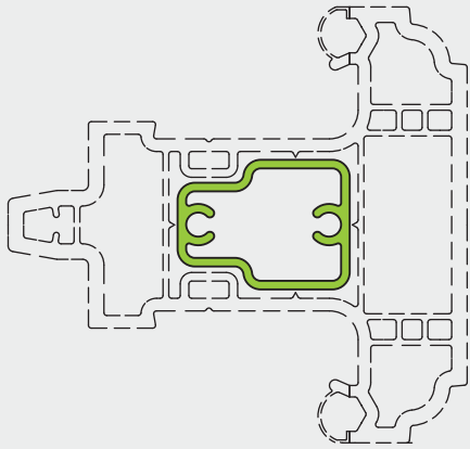
LFS212 80mm Flush Sash Transom Aluminium Reo
