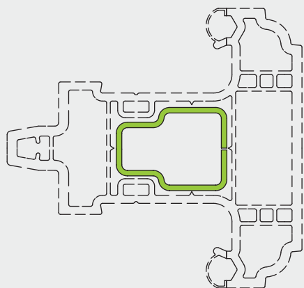
LFS121 80mm Flush Sash Transom Steel Reo
