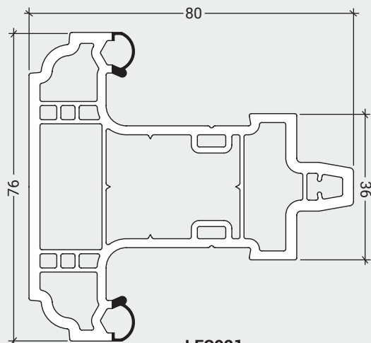
LFS021 80mm Flush Sash Transom T
