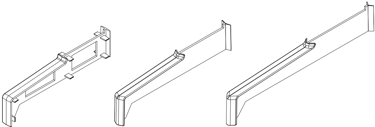
LMO354 In-line jointer (150mm cill ONLY) LMO355 135° jointer (150mm cill ONLY) LMO356 90° jointer (150mm cill ONLY)
