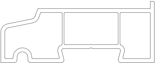
LSL085 85mm Cill
