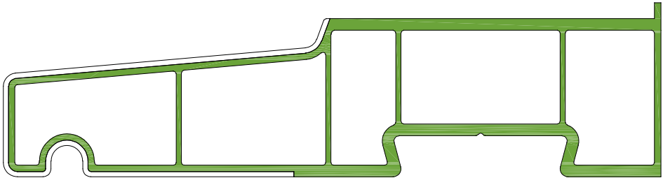
LSL125 125mm Cill
