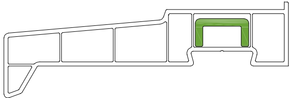
LAN165 PVCu Cill Reinforcement
