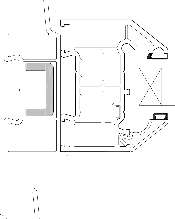
Section 'D-D'
