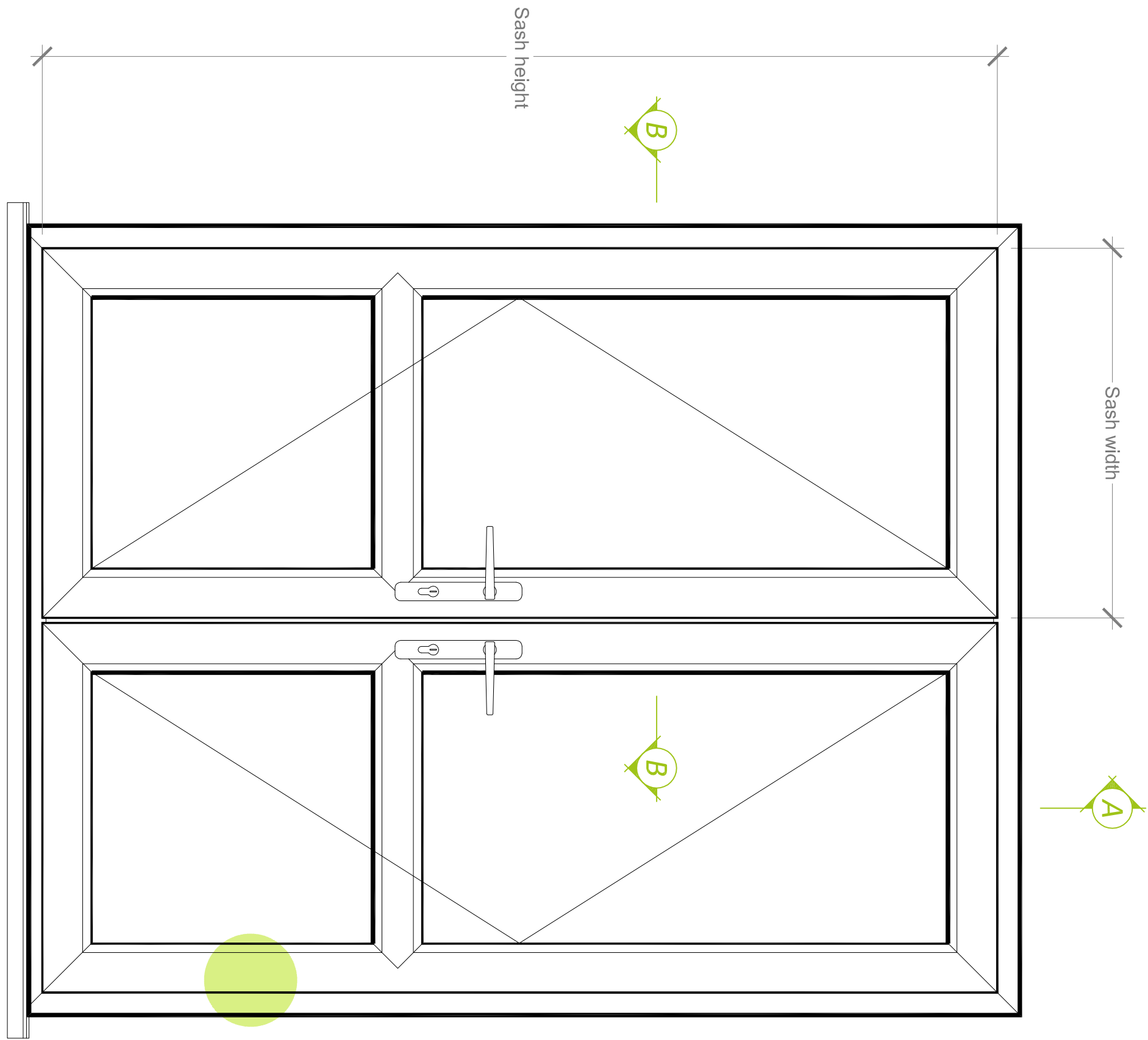
Typical Elevation Viewed from Outside Scale 1:10
