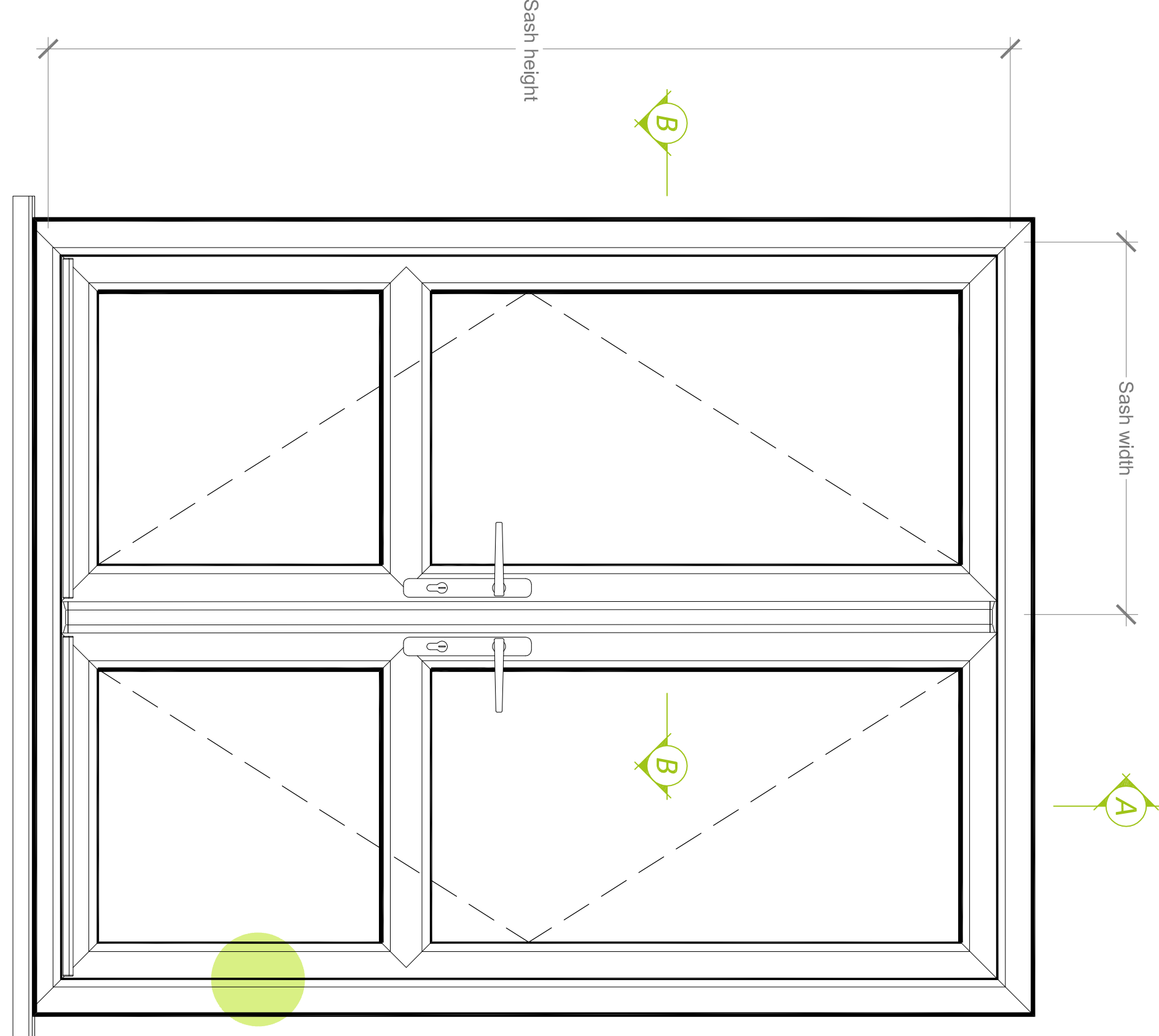
Typical Elevation Viewed from Outside Scale 1:10
