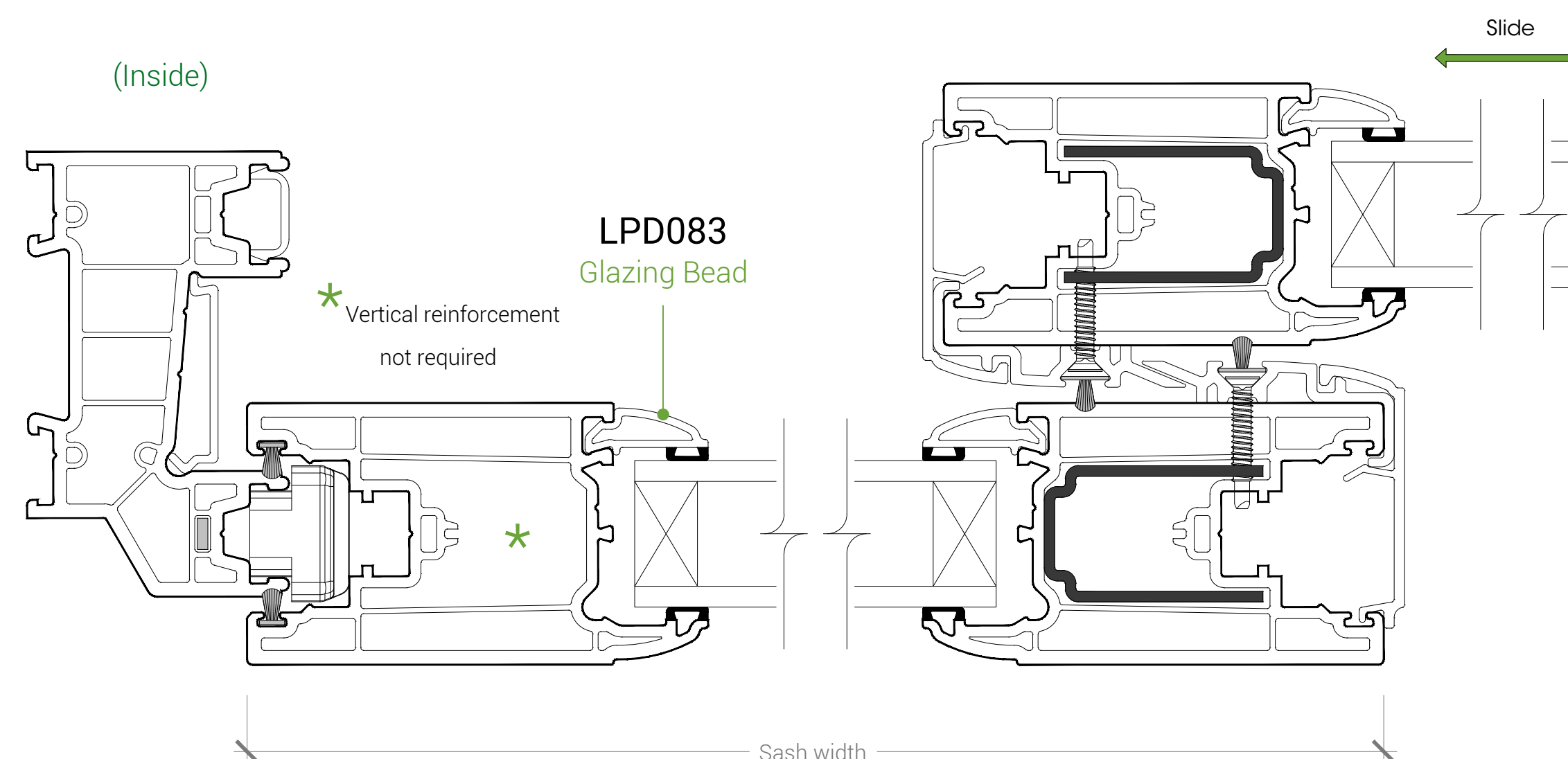
SECTION 'C-C'
