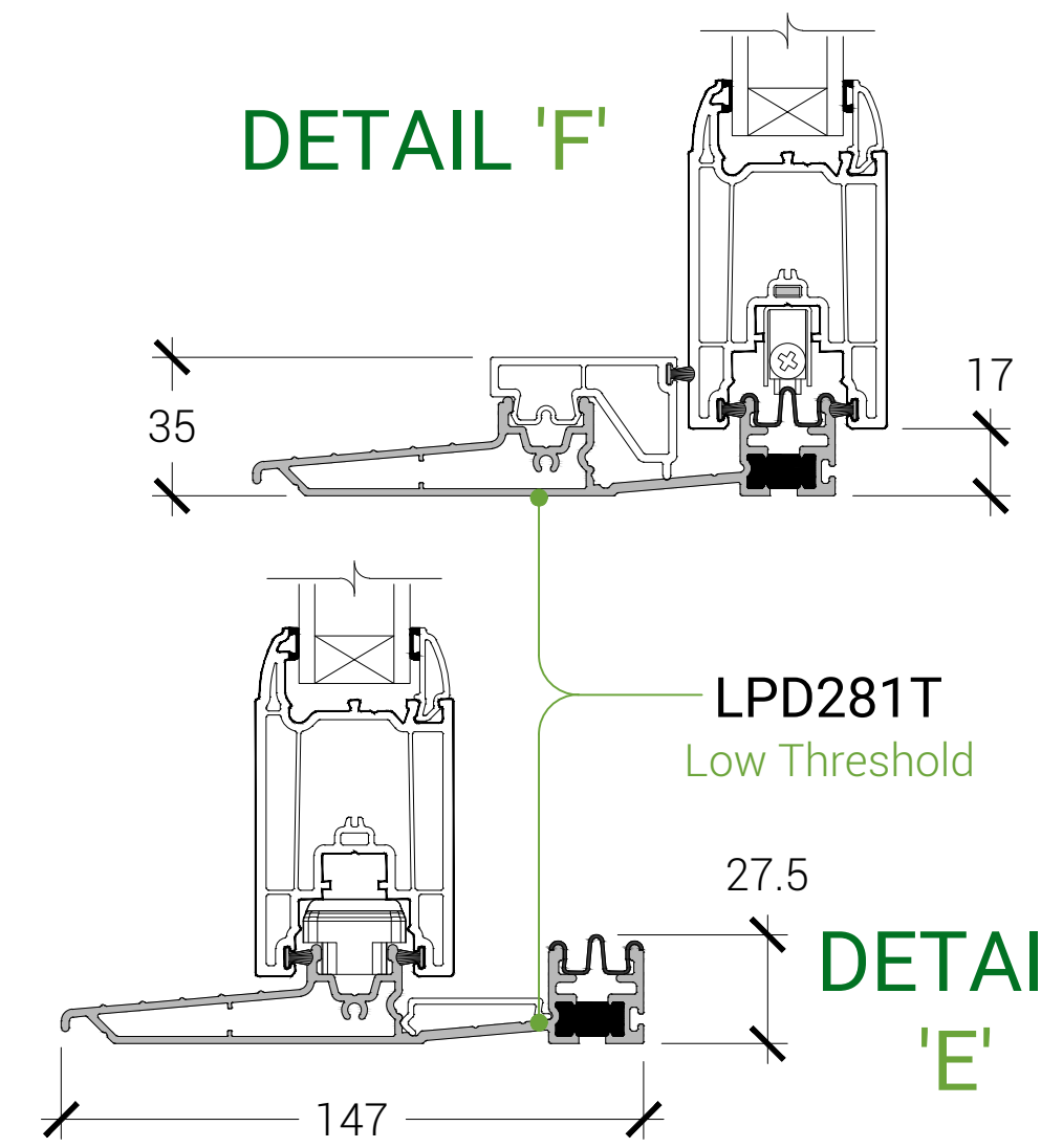
DETAIL 'F'
