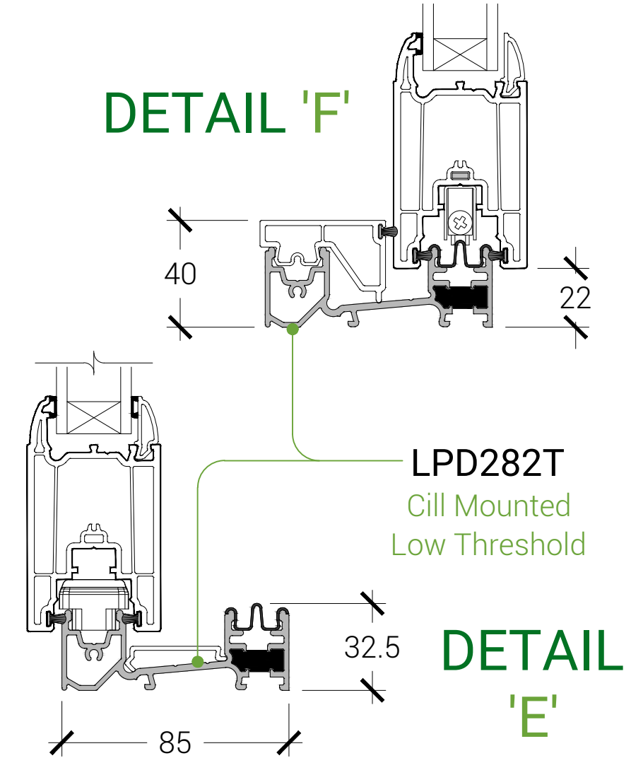
DETAIL 'E'
