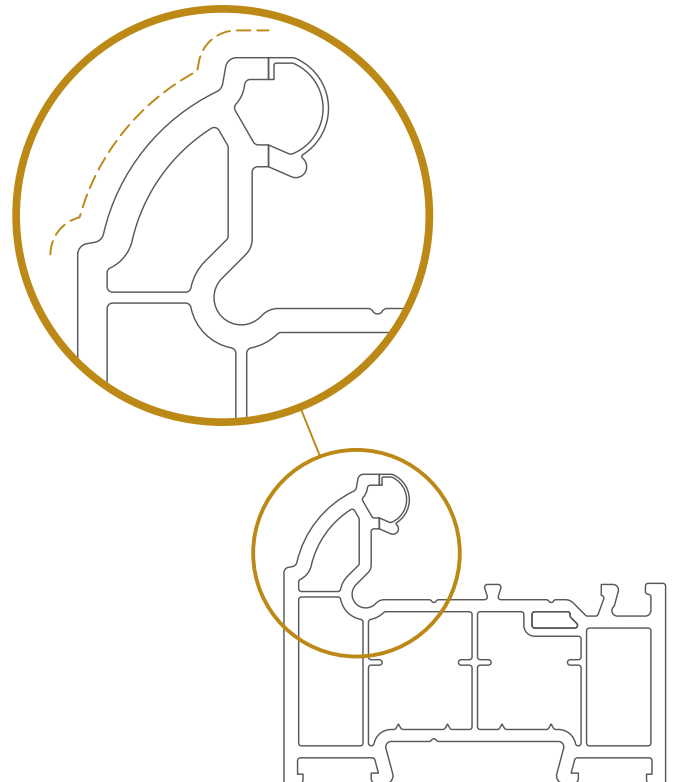
Example profile shown is LSW01 I LSW - Liniar 'Sculptured' Window
