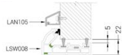
ULTRA SLIM U-PVC THRESHOLD
