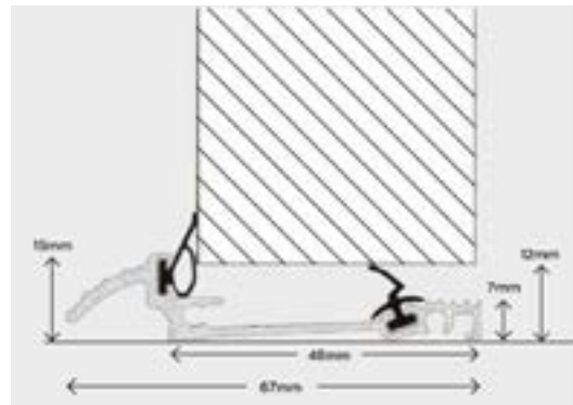
LOW ALUMINIUM THRESHOLD PART M COMPLIANT
