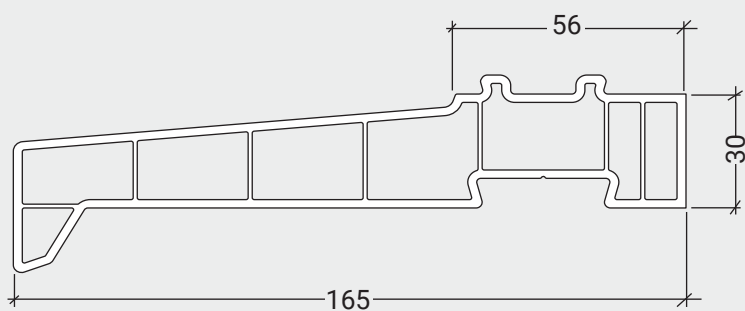
LCL165 165mm Cill
