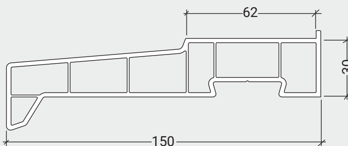
LSL150 150mm Cill
