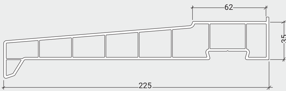
LSL225 225mm Cill
