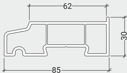
LSL085 85mm Stub Cill
