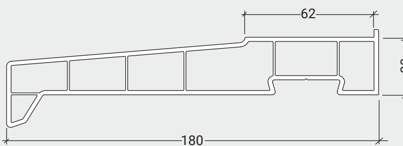
LSL180 180mm Cill
