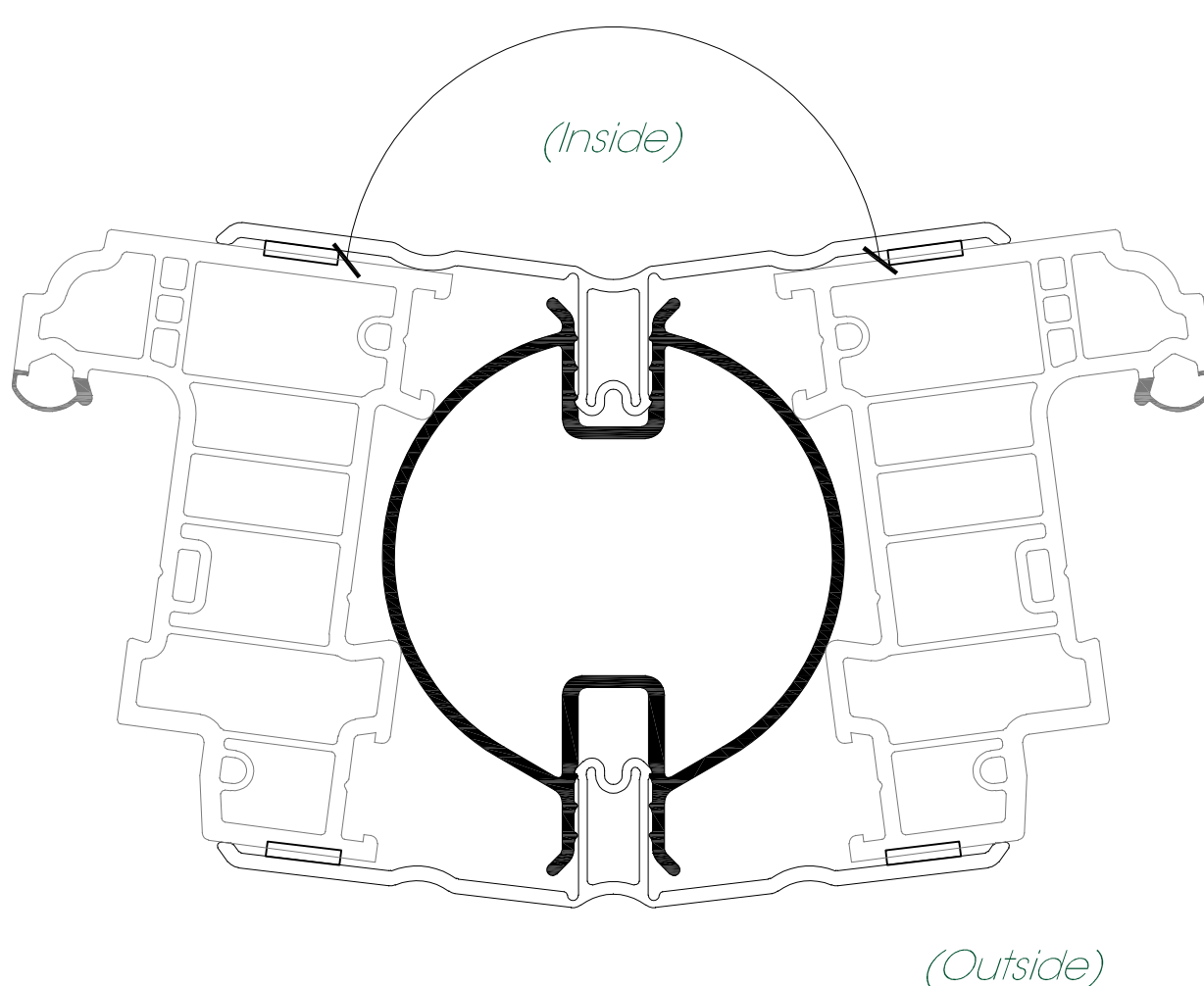
LFS232 Large Bay Pole
