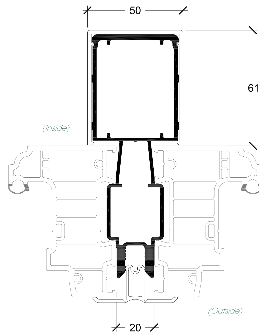
LAN214 Structural Joint
