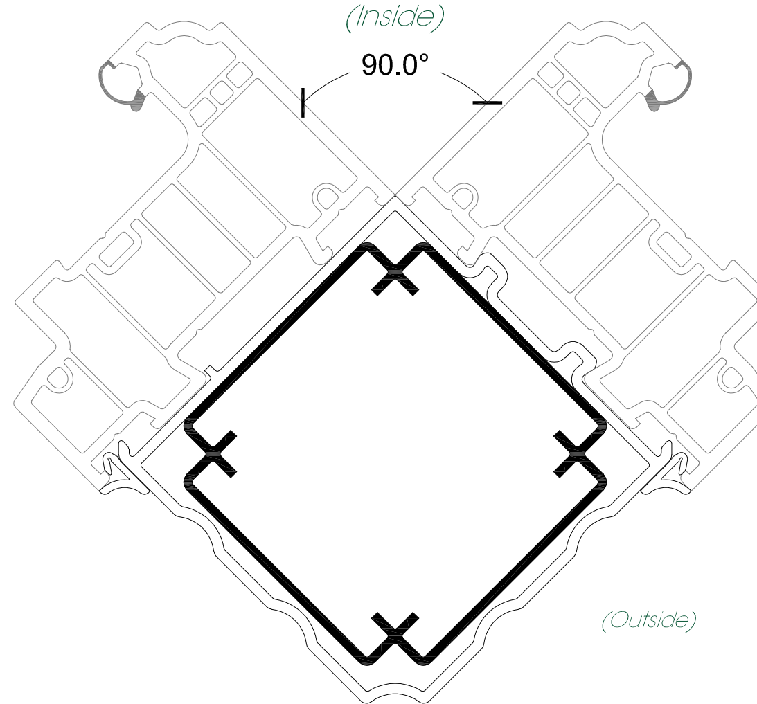
LAN253 90° Corner Joint
