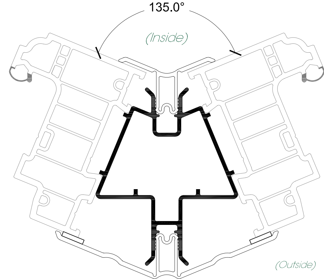
LFS251 135° Corner Joint
