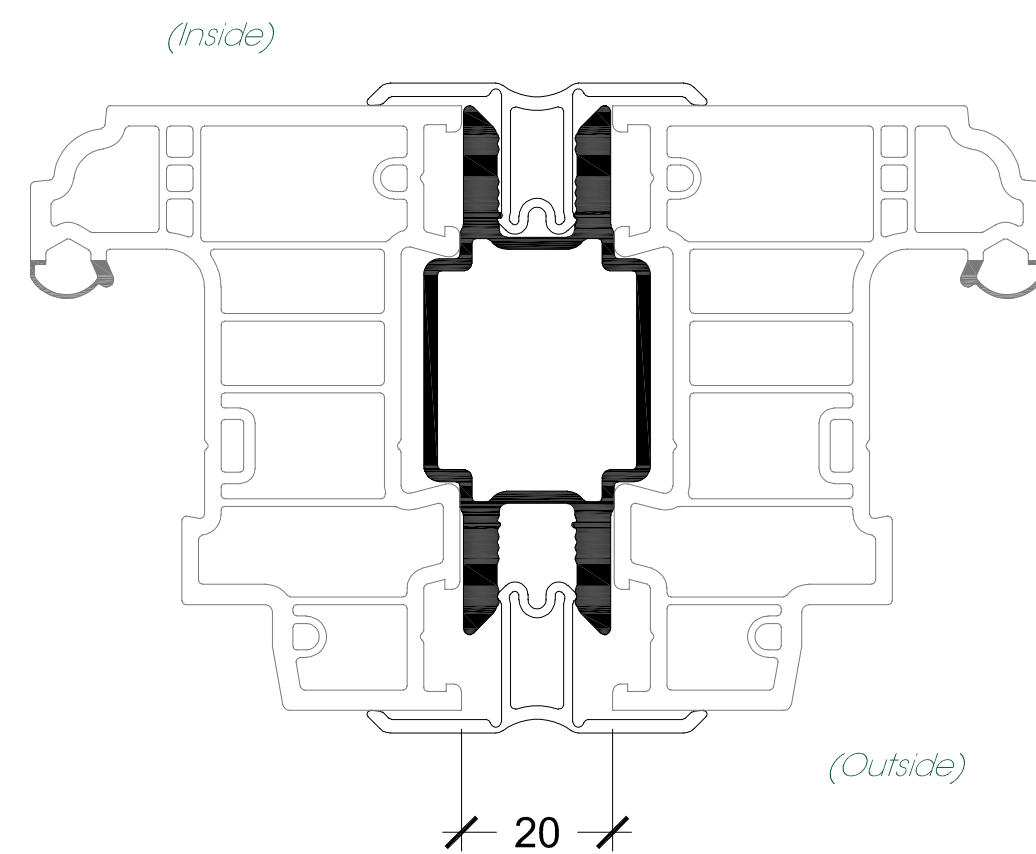
LAN212 Medium Duty Butt Joint
