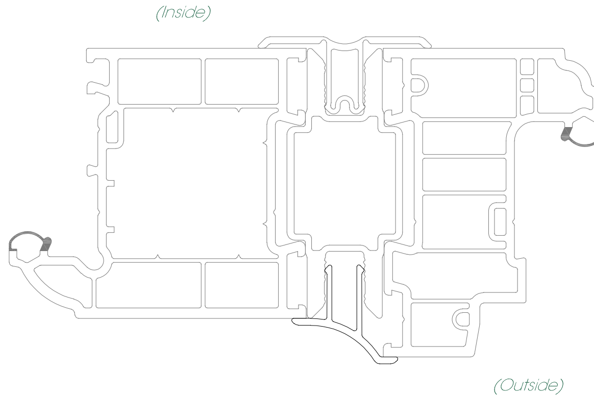
LFS102 70mm to 80mm Joint trim
