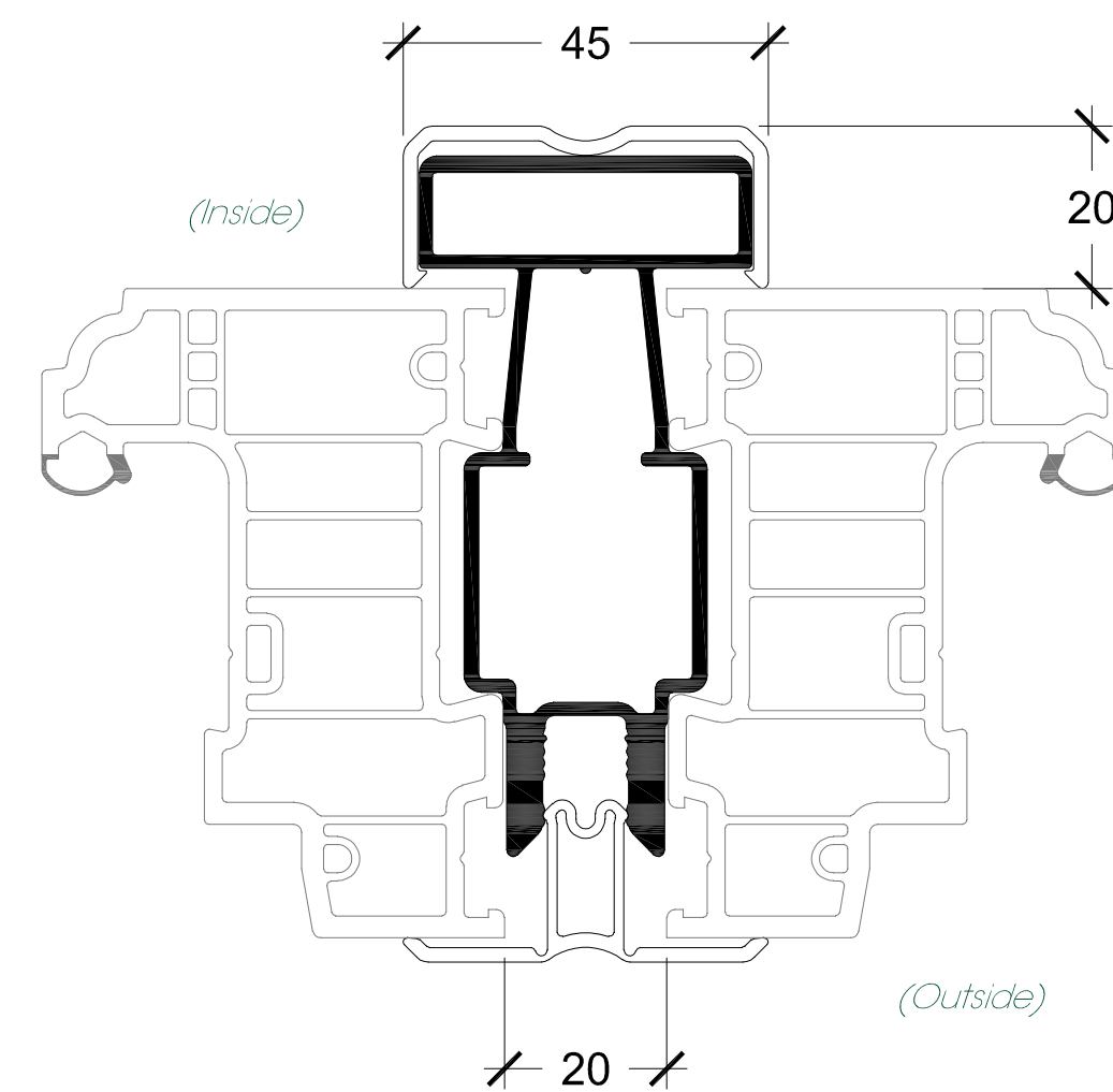
LAN213 Heavy Duty Butt Joint
