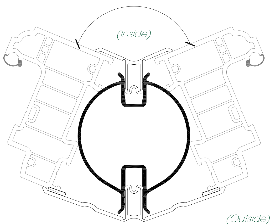
LFS232 Large Bay Pole
