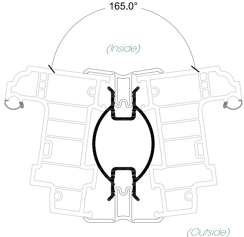
LAN233 Bow Pole
