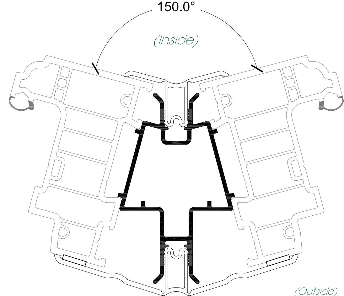
LFS252 150° Corner Joint
