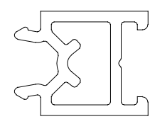
LAN146 20mm Universal Frame Extension
