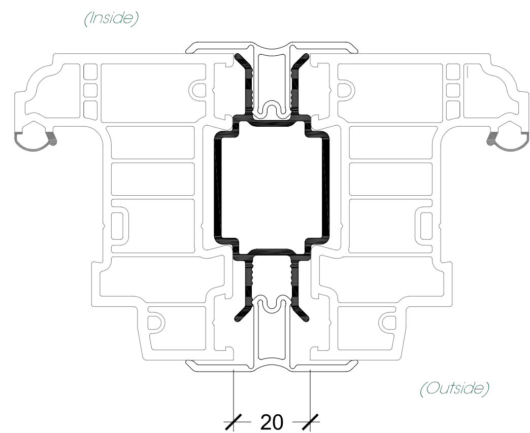
LAN211 Standard Butt Joint
