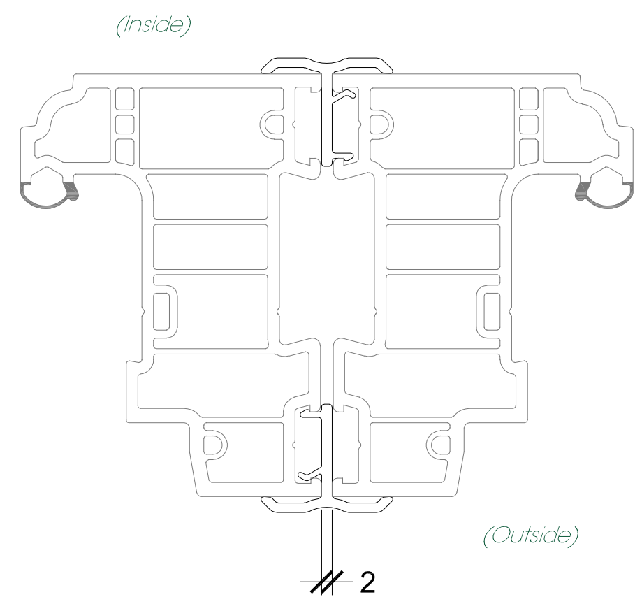
LAN103 Single Butt Joint
