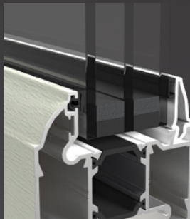
36MM TRIPLE GLAZING
