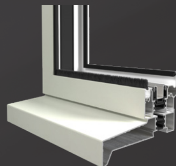
FRAME & CILL HEIGHT: 92mm (inc. cill)
