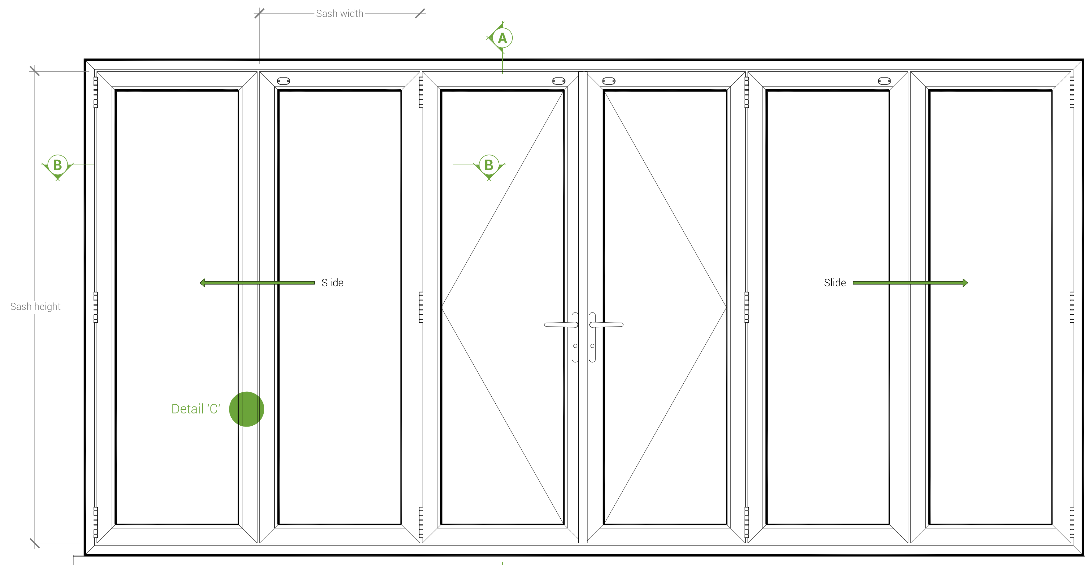
TYPICAL ELEVATION Viewed from Outside Scale 1:10
