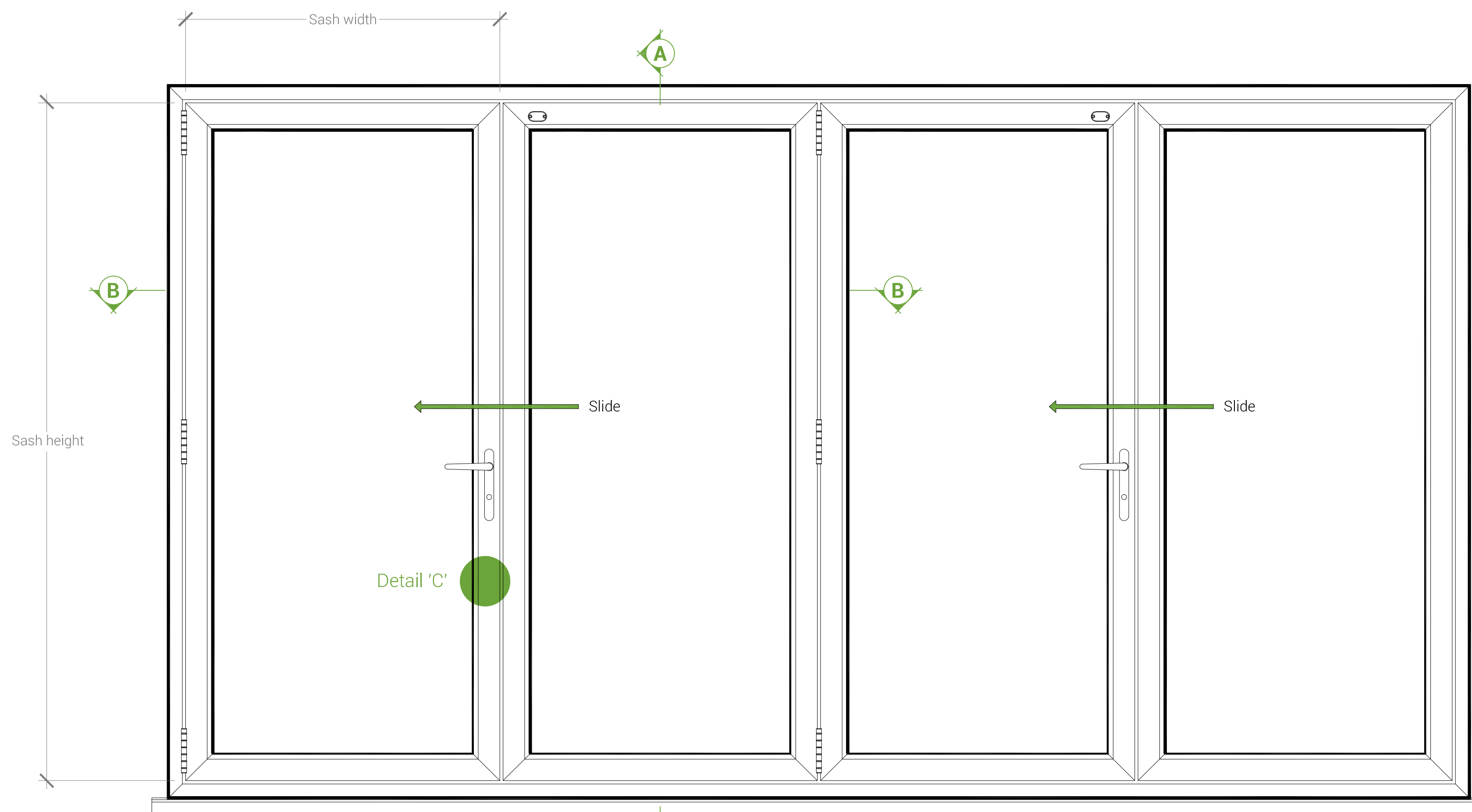
TYPICAL ELEVATION Viewed from Outside Scale 1:10
