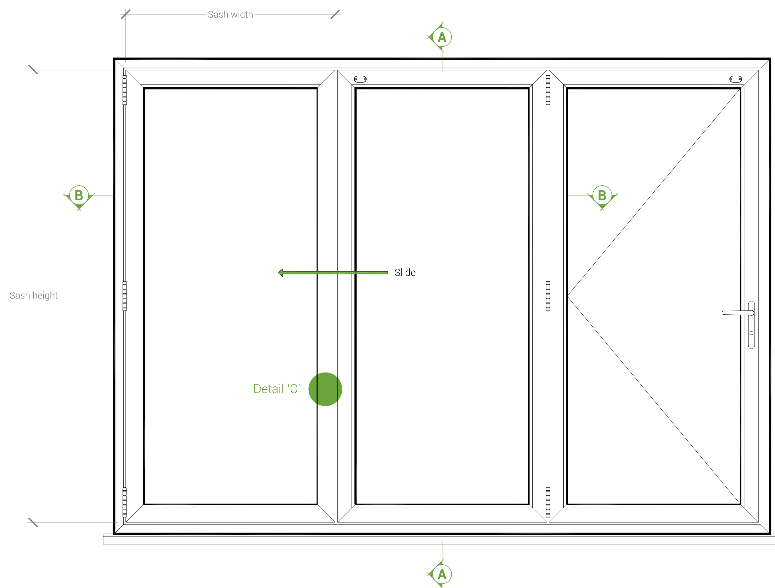
TYPICAL ELEVATION Viewed from Outside Scale 1:10
