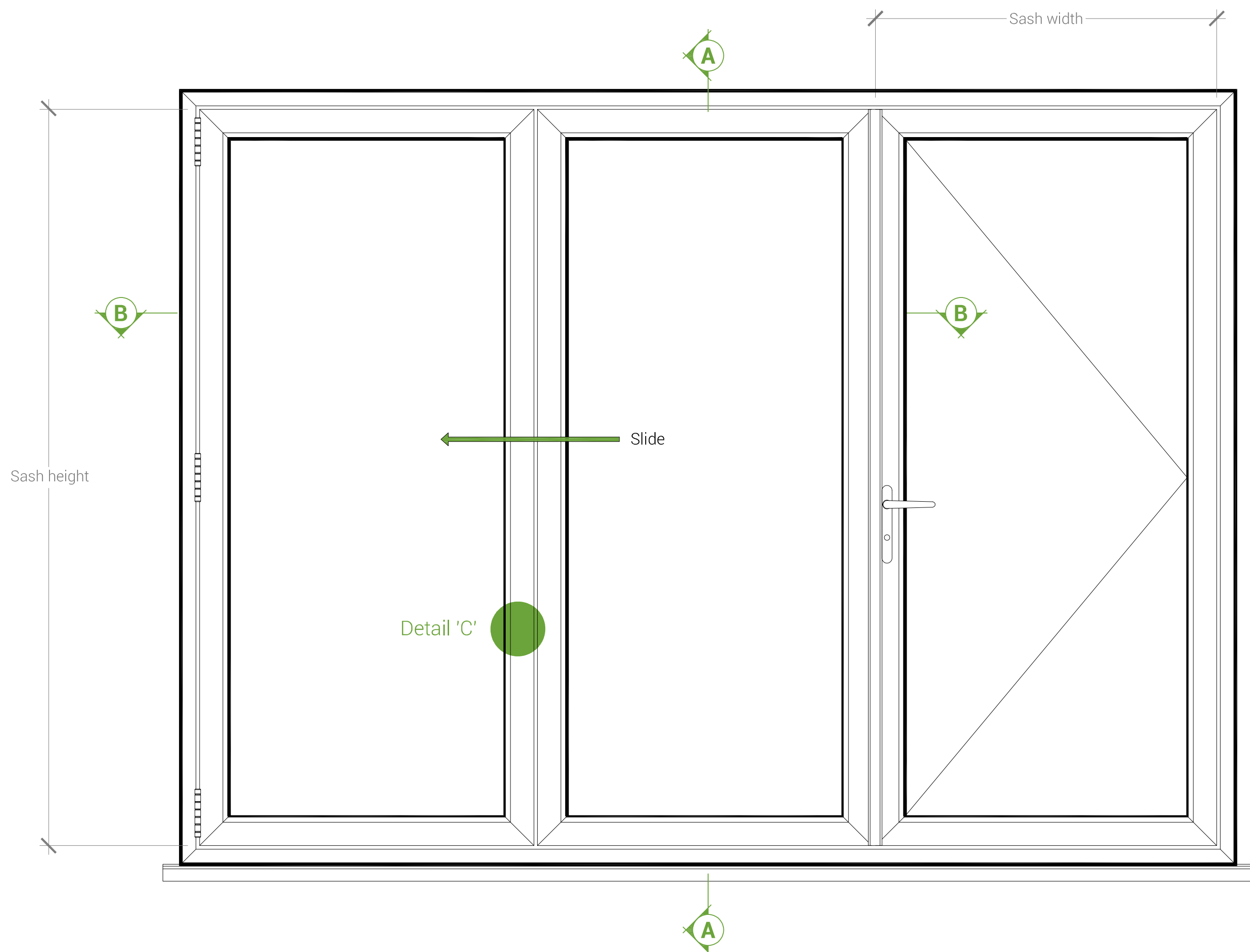
TYPICAL ELEVATION Viewed from Outside Scale 1:10
