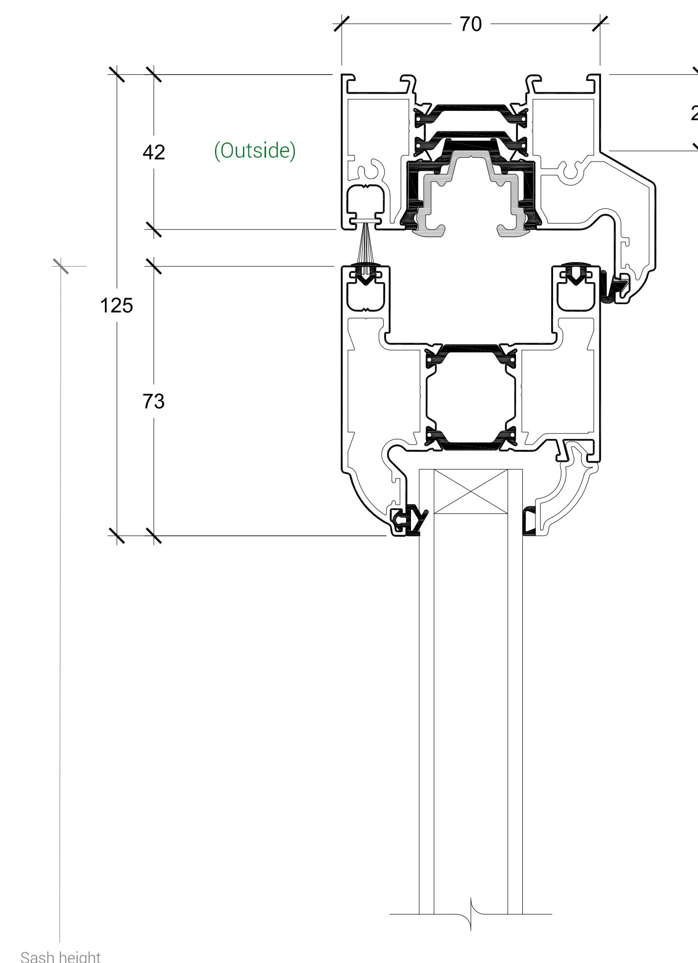
Sash height
