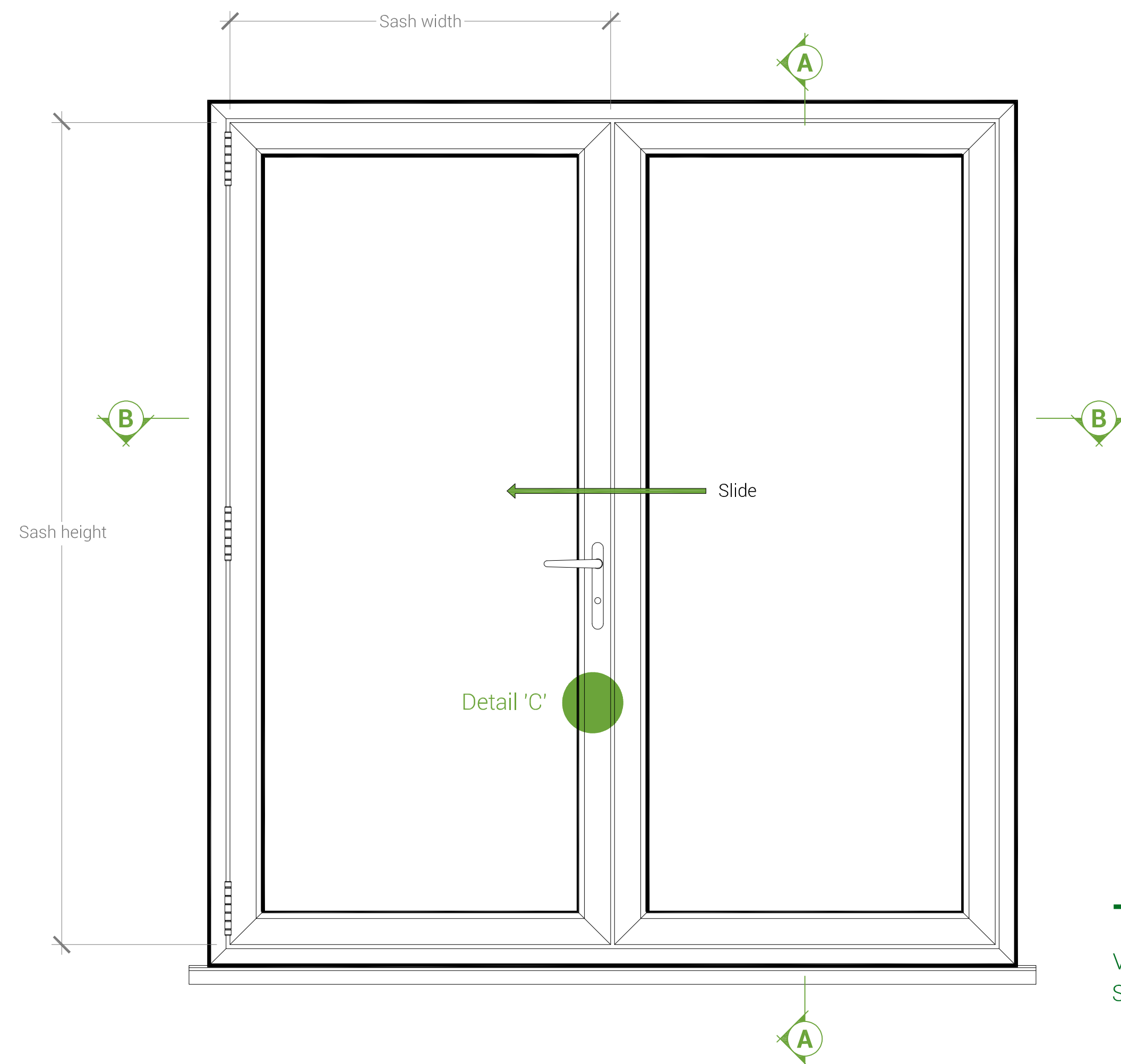
TYPICAL ELEVATION Viewed from Outside Scale 1:10
