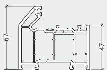
LCW018 44mm Composite Door Outer Frame
