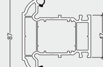
LSW026 Intermediate Transom T
