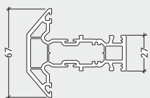
LCC021 48mm Composite Door Transom T
