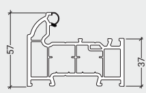
LSW011 Main Frame
