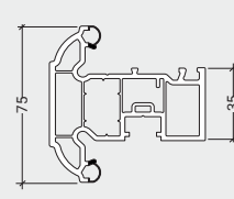
LSW031 Sash T
