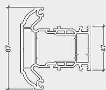
LSW028 44mm Composite Door Transom T
