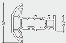
LSC021 48mm Composite Door Transom T
