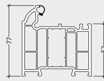
LSW017 EnergyPlus Large Main Frame
