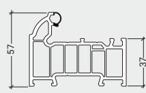
LSW012 EnergyPlus Main Frame
