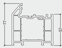
LCC016 48mm Composite Door Outer Frame
