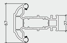
LSW021 Transom T
