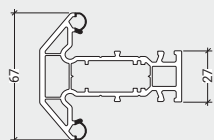
LCW021 Transom T
