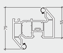
LCW032 Sash Z
