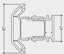
LCW028 44mm Composite Door Transom T
