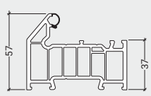
LCW012 Energy Plus Main Frame
