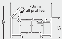
LCW011 Main Frame
