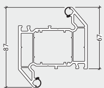
LCW027 Internal Transom Z
