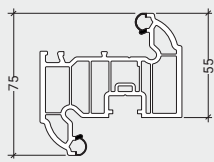
LSW032 EnergyPlus Sash Z
