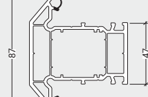
LCW026 Internal Transom T
