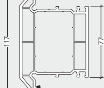
LCW029 Midrail
