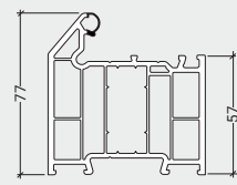
LCW017 EnergyPlus Large Main Frame
