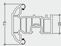
LSW033 EnergyPlus Sash T
