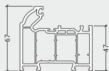
LSW018 44mm Composite Door Outer Frame
