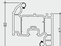
LSW035 T&T Sash
