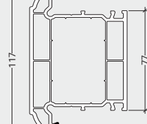
LSW029 Midrail
