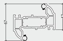
LSW022 Transom Z
