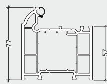
LSW016 Large Main Frame
