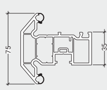
LCW031 Sash T
