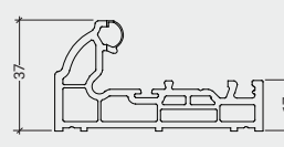
LSW010 Sculp PVCu Threshold
