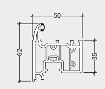
LSW030 Flush Sash
